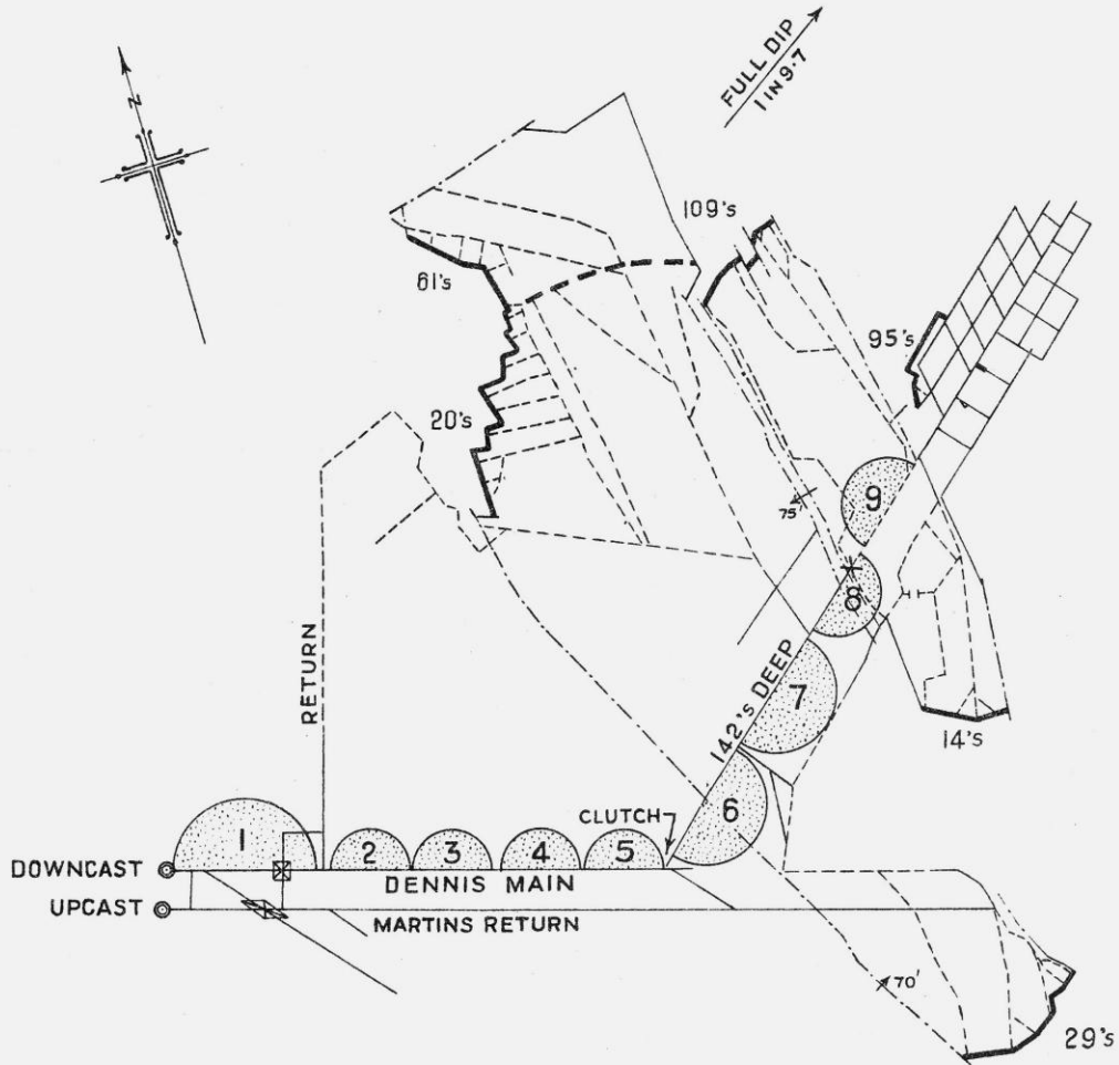
PLAN INDICATING ZONES FROM WHICH DUST SAMPLES WERE COLLECTED ON DENNIS MAIN AND 142's DEEP HAULAGE ROADS.
